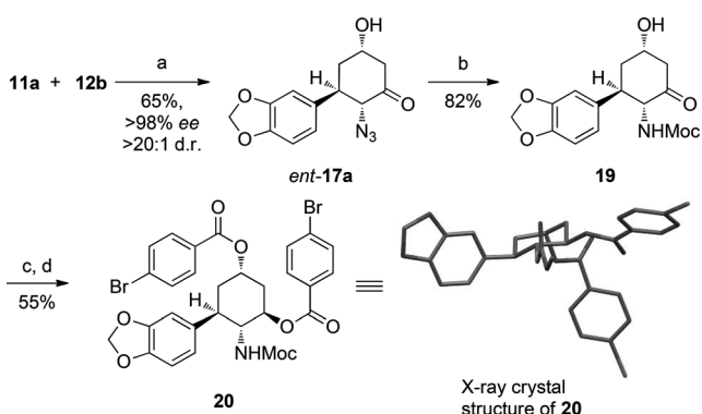
Scheme 3. Reagents and conditions: Yields of isolated products are indicated. [11] a) 13d (10 mol%) and 16a (10 mol%), CH 2 Cl 2 , RT, 24 h, 65%. b) DMDC (3.0 equiv), H 2 , 10% Pd/C (0.075 equiv), 50 psi, MeOH, RT, 16 h, 82%. c) Me 4 NHB(OAc) 3 (4.0 equiv), acetonitrile/AcOH (96:4), RT, 12 h, 77%. d) p -BrBzCl (3.0 equiv), DMAP (0.10 equiv), py, 0°C, 8 h, 71%. Bz = benzoyl, DMAP = 4-dimethylaminopyridine, DMDC = dimethyl dicarbonate.
